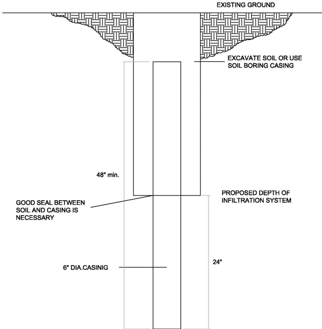
Figure 2. Encased Falling Head Schematic
